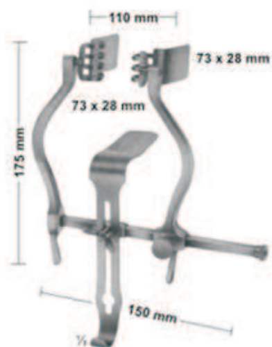
09-101 JUDD-MASSON Bladder and suprapubic retractor
