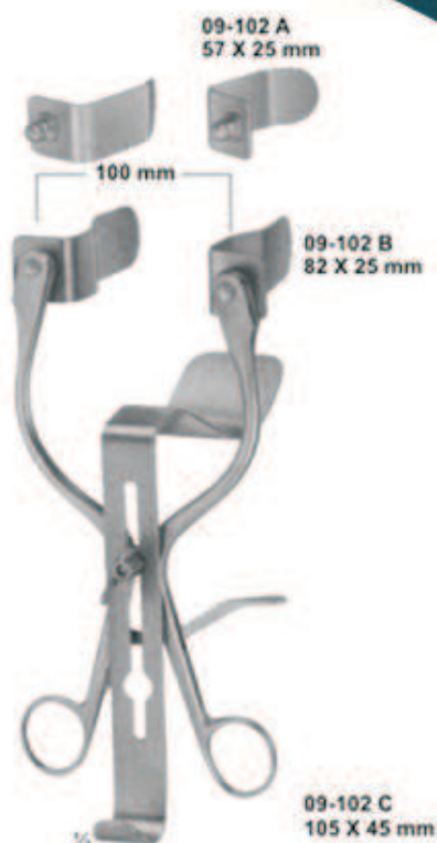
09-103 MILLIN Bladder retractor, complete 105X45 mm
